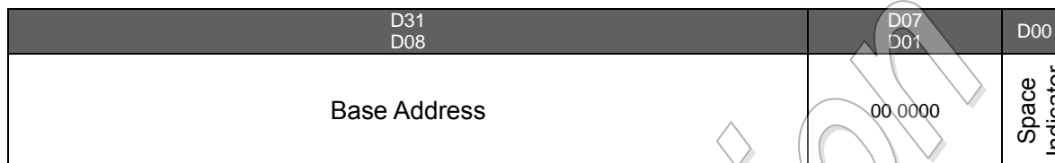
Figure C- 4 : PCI Config. Base Address Register for 256Byte Register Map
