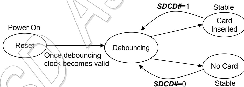
Figure 2-10 : Card Detect State
