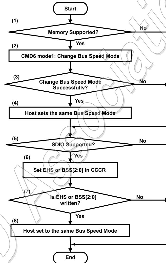
Figure 3-19 : Bus Speed Mode Setting for Combo Card
